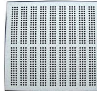
RAF-PP 001 Perforated Panel 17% Ventilation Rate
